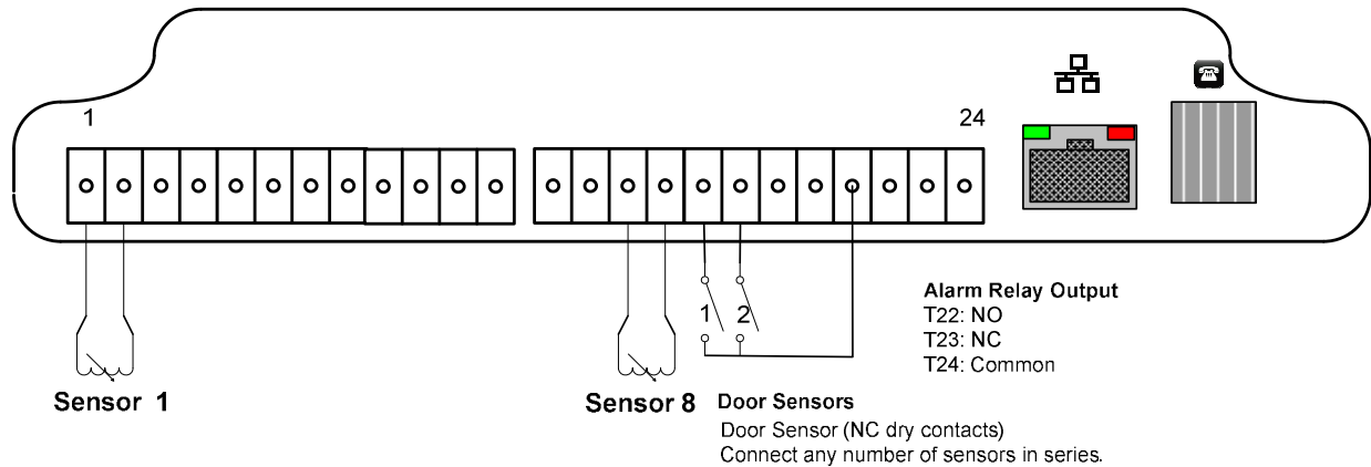
Wiring Diagram (side view of enclosure)
